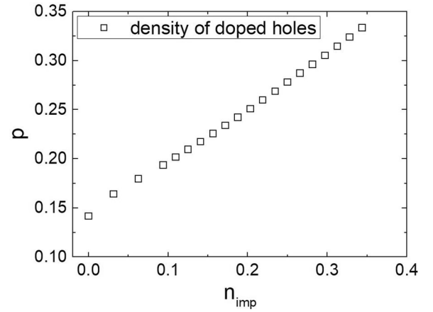
Fig. 2 Plot of the density of doped holes as a function of impurity concentration. The disorder strength is fixed with w = 1 .
